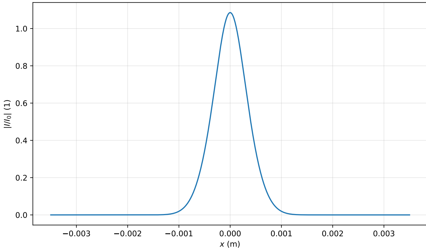
Intensity profile I(x, y = 0, z = 0.478m)/I_0 , P_{in}=0.7P_{cr} , artificial time
